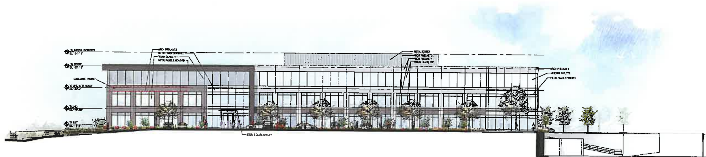
1 CONCEPTUAL EAST ELEVATION- BUILDING C 1/16"=1'-0"
